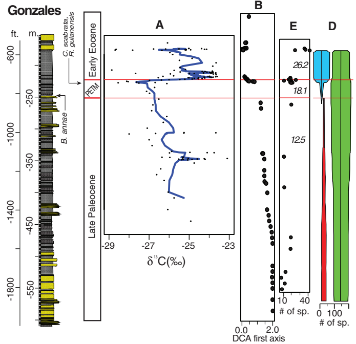
restricted taxa (red), whereas diversity of taxa that cross from the Paleocene into the PETM (green) does not change. Increase in diversity at the onset of the PETM is due to a large addition of taxa to the preexisting Paleocene flora. (E) Within-sample (rarefied) diversity at a count of 100 grains. The PETM (mean = 18.1) is more diverse than the Paleocene (12.5) and less diverse than the Eocene (26.2).
